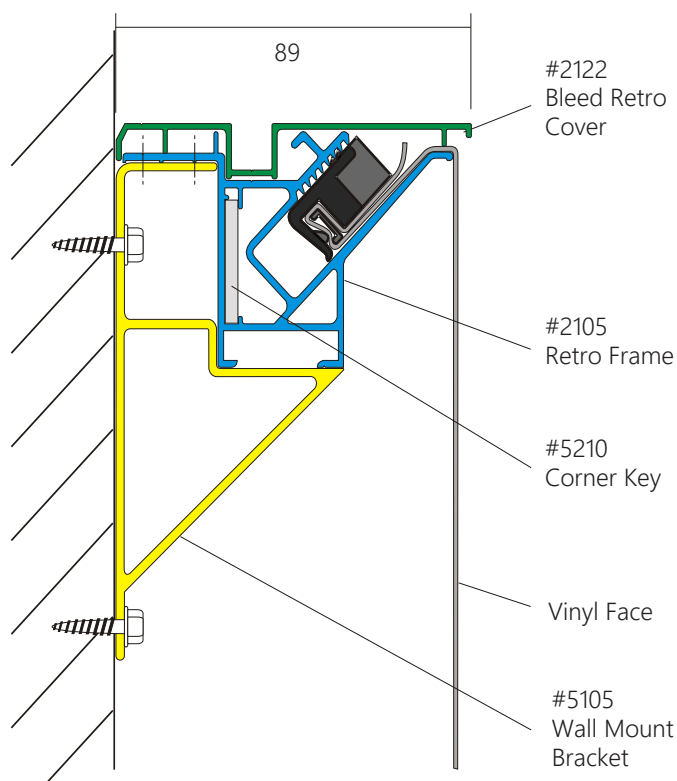
Assembly using #5105 Wall Mount Bracket
