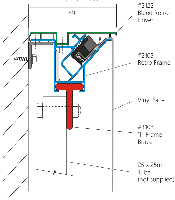
Assembly using #3108 "T" Frame Brace
